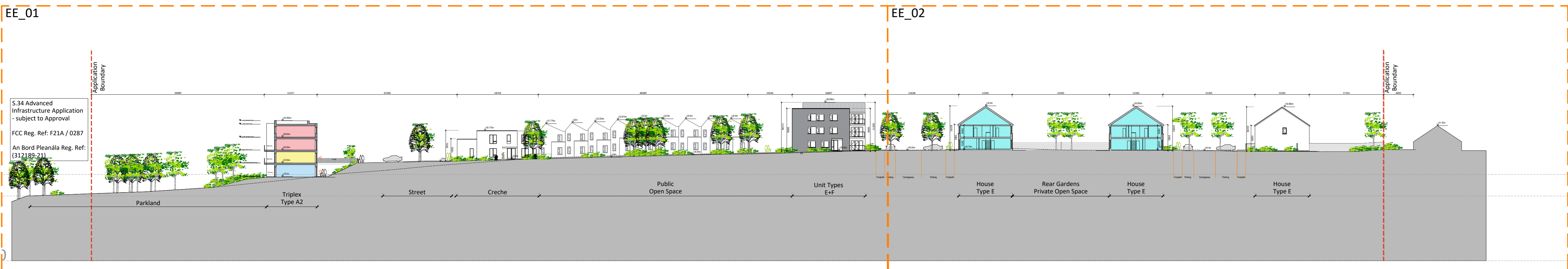
Section EE Esc 1:500
